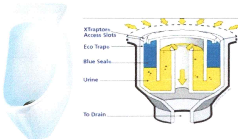
Waterless Urinal
